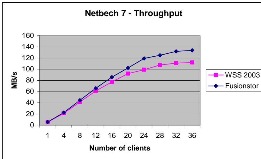
Figure 2: Throughput at variable client numbers
