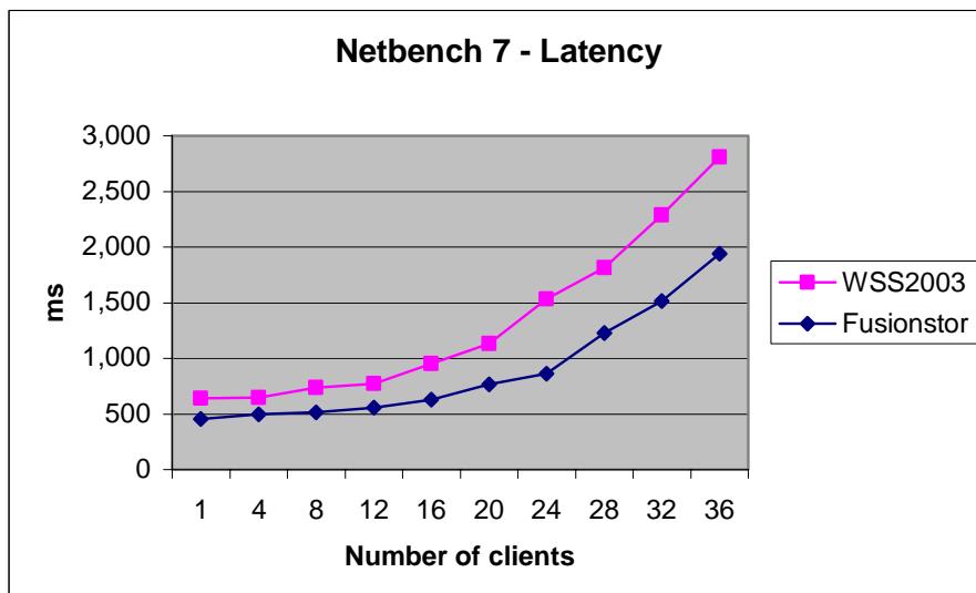
Figure 3: Latency at variable client numbers
